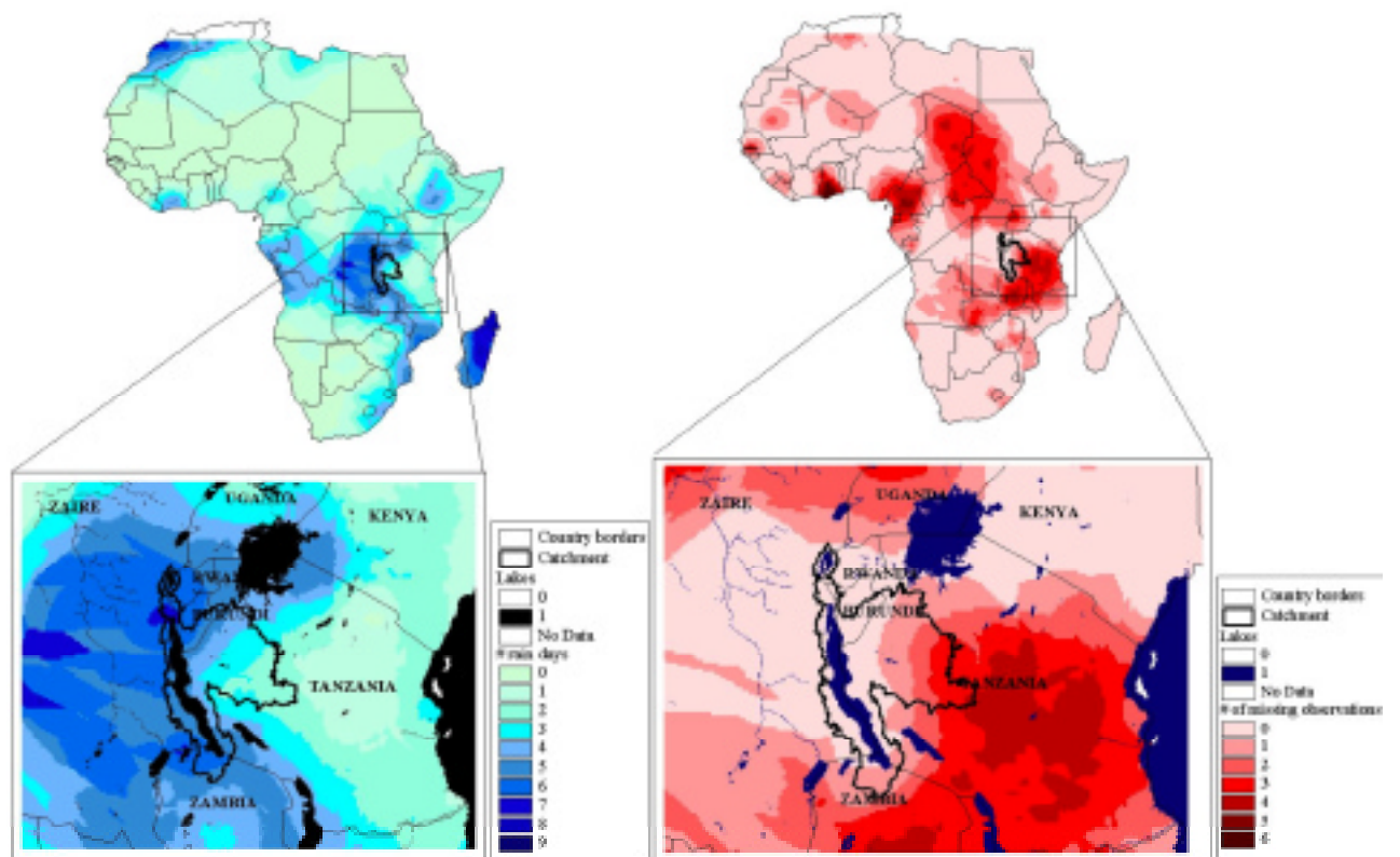
Figure 8. The number of rain days per decad calculated from the GTS station data. Left) Interpolation of rain days using kriging. Right) Interpolation of the missing data in each decad using kriging.
