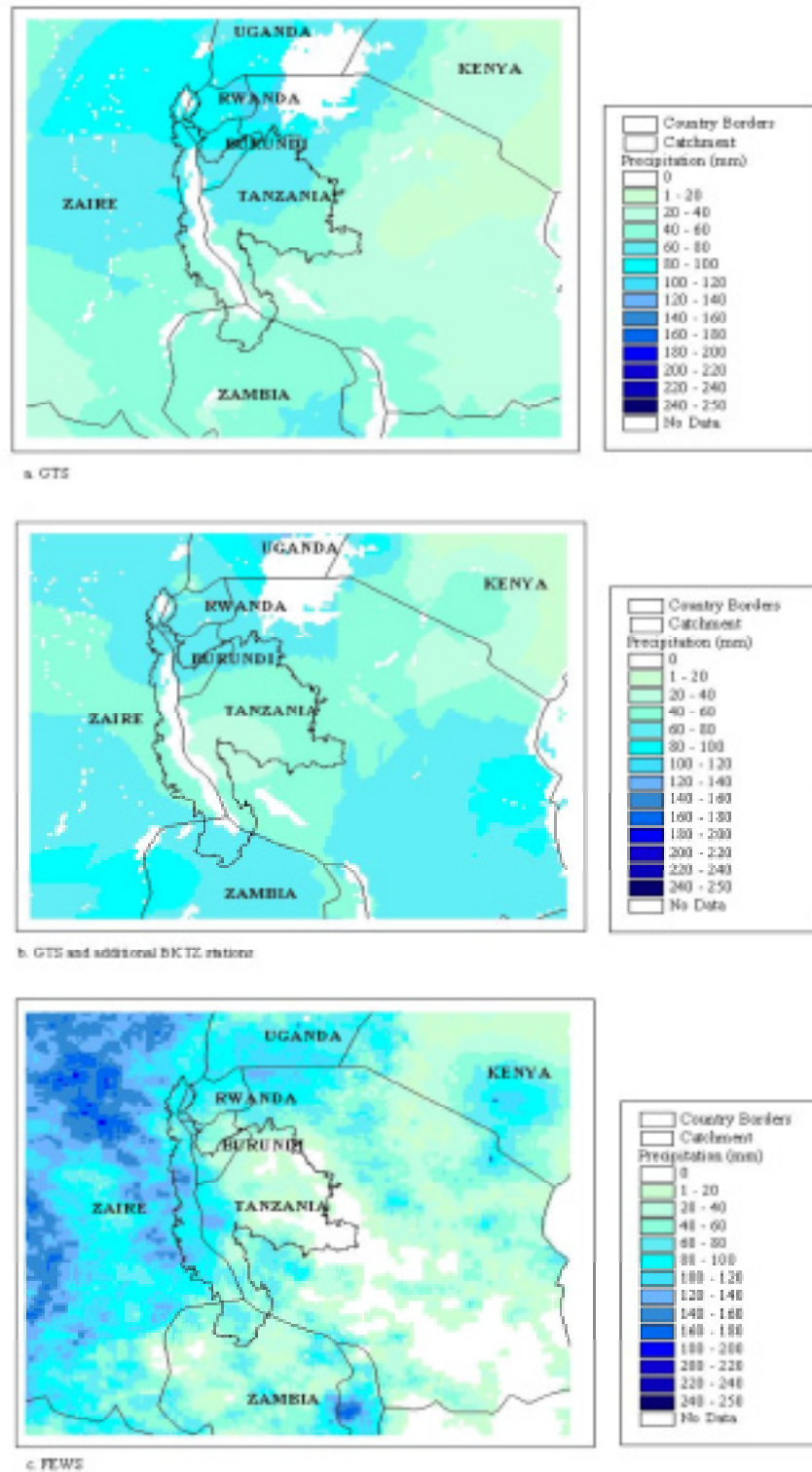
Figure 11. The Lake Tanganyika catchment shown in more detail. FEWS and interpolated GTS data for the second decad of March 1996.
