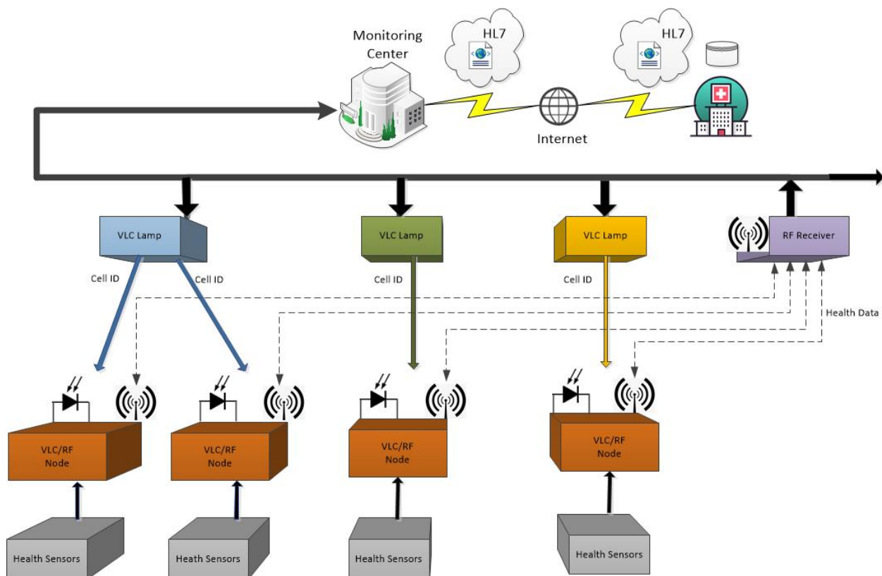
Figure 2. Network architecture.
