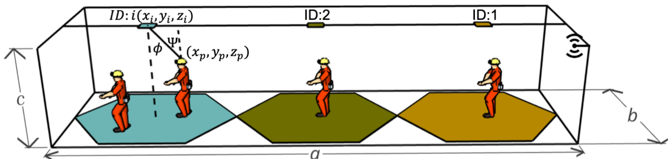
Figure 4. VLC Downlink.
